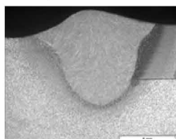
HQ-weld-seam
